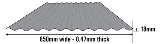
Sheet Profile Corrugated
